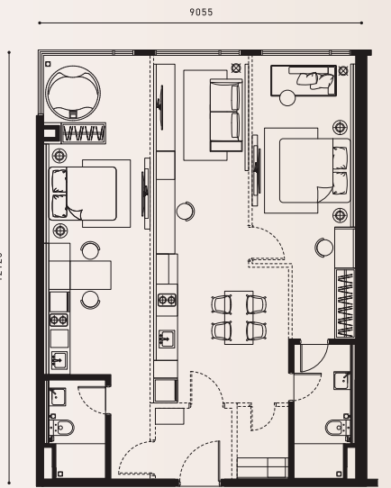
SOVO E UNIT AREA 109.81M 2 | 1182FT 2
