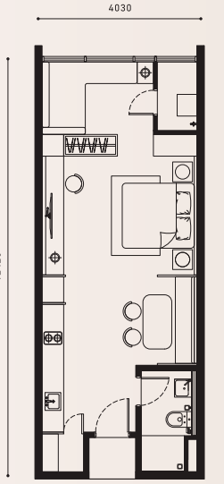
SOHO B UNIT AREA 50.00M 2 | 538FT 2
