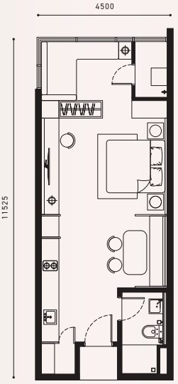
SOHO A (CORNER) UNIT AREA 51.86M 2 | 558FT 2
