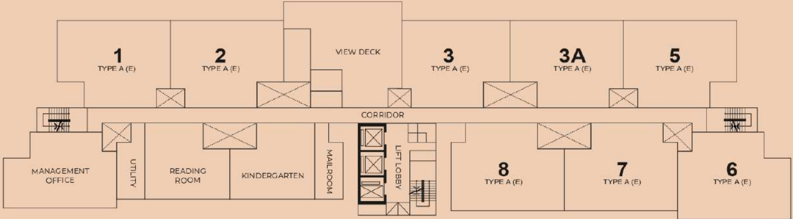
Level 1
