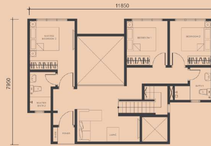
PENTHOUSE UPPER FLOOR PLAN
